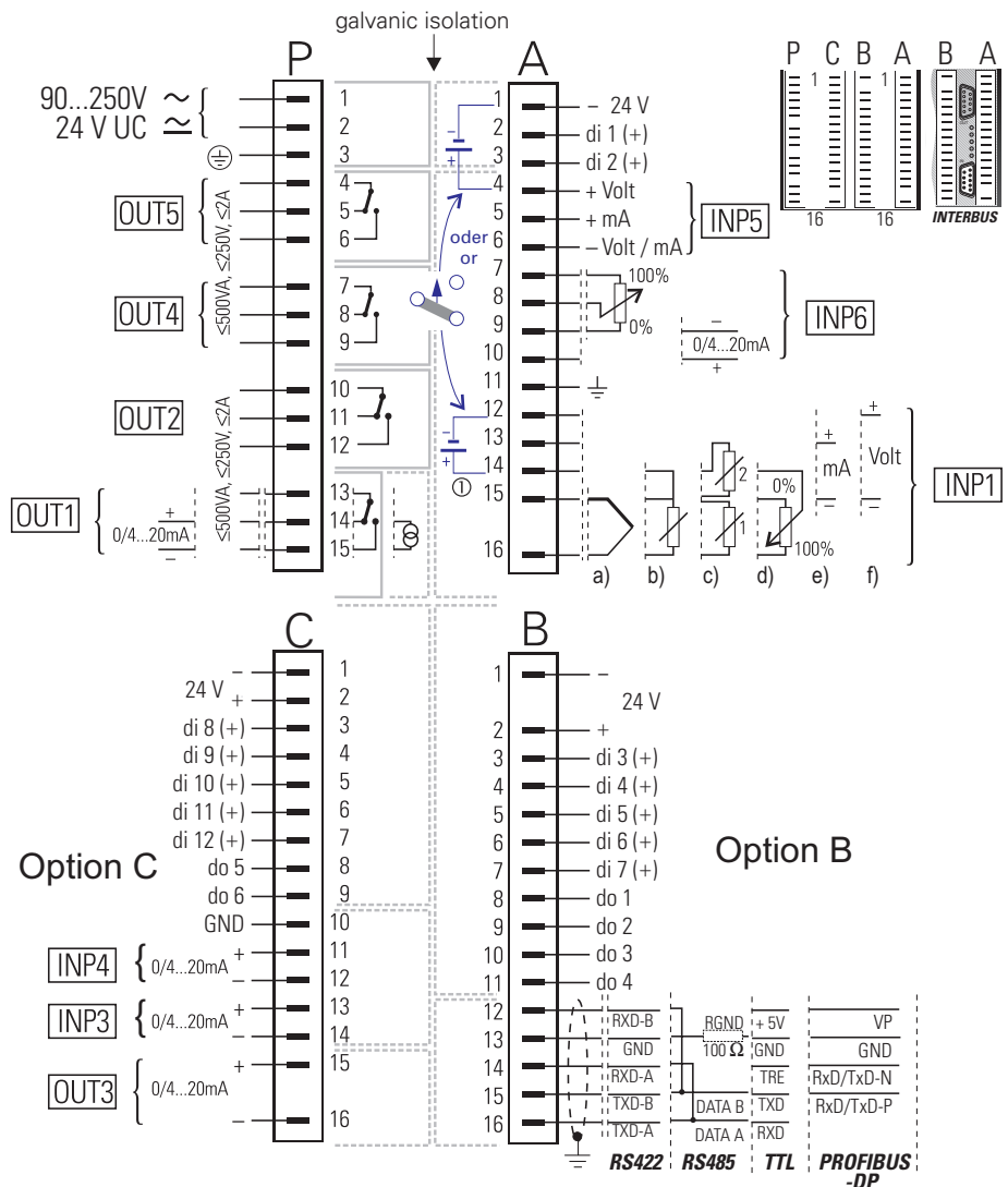
Fig. 1 Electrical connections
